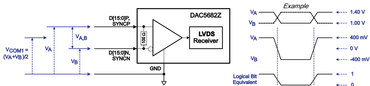
Figure 41. LVDS Data (DxP/N, SYNC/N Pairs) Input Levels
