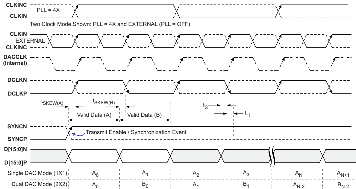
Figure 33. Clock and Data Timing Diagram
